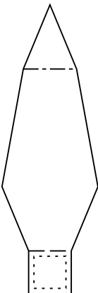
R16 | cut 1 18.00 x 54.00 mm
