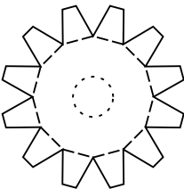
R27 | cut 1 18.00 x 44.00 mm
