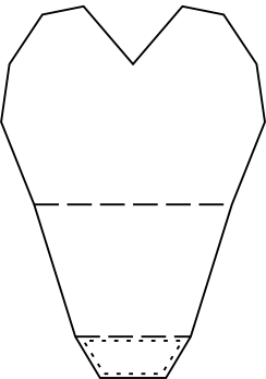
P3 | cut 1 32.00 x 45.00 mm
