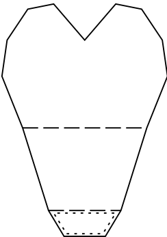
P1 | cut 1 32.00 x 45.00 mm
